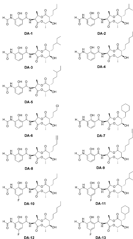
Figure 2. Structurally characterized C8-deacylated variants of ANTs.
